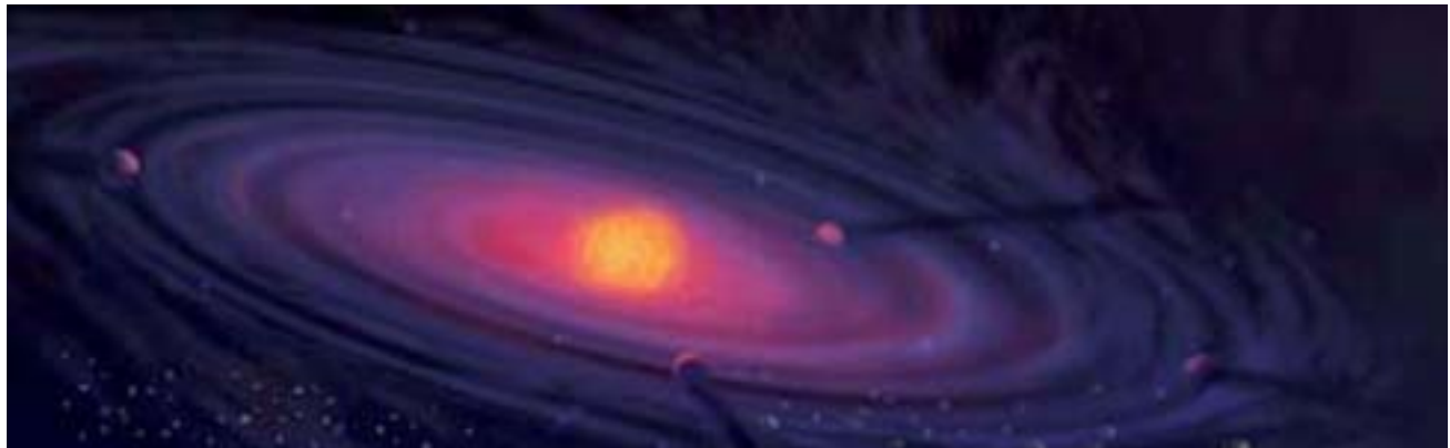
Circumstellar Debris Disk. CREDIT: NASA
