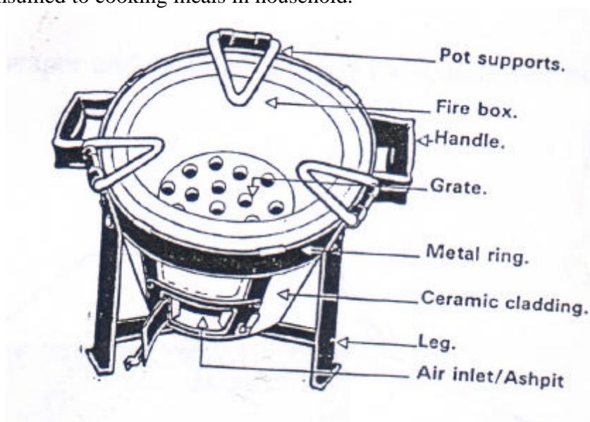
Figure 1: Different parts of Sazawa charcoal stove.
